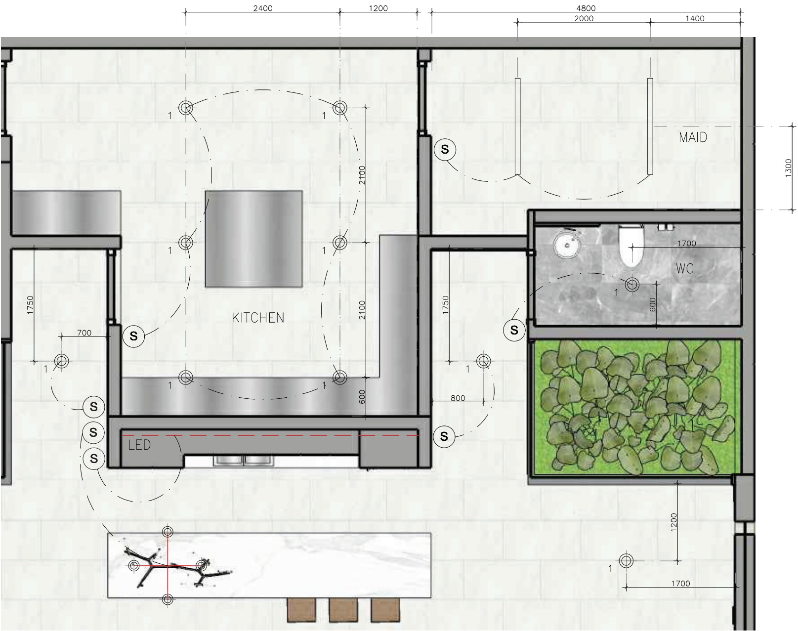
LIGHTING SYSTEM SYMBOLS RECEPTACLE,TV.OUTLET&TELEPHONE OUTLET SYMBOLS
