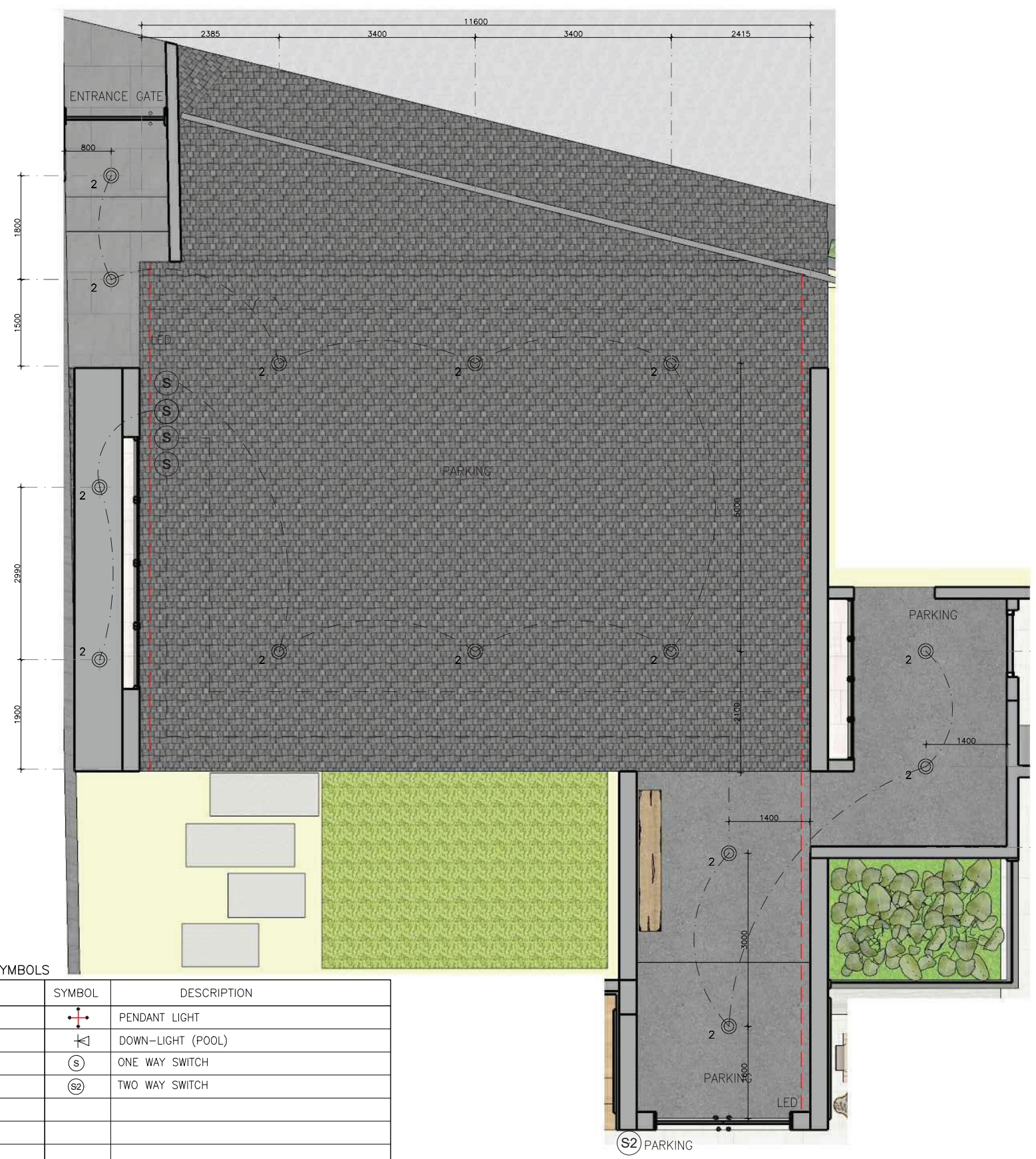
1ST LIGHTING PLAN SCALE 1:75
